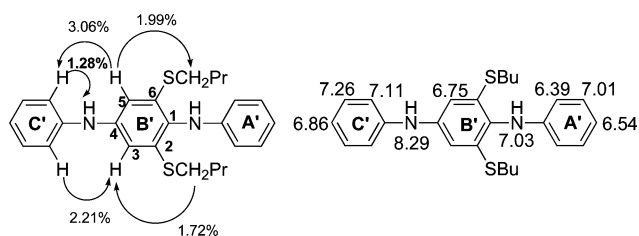
Fig. 6 The NOE results of 2,6-diPDA and its peak assignments.
