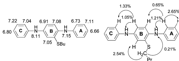
Fig. 3 The NOE results of mono-PDA and its peak assignments.
