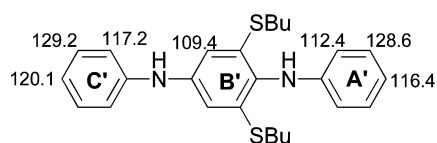
Fig. 7 The ^{13}\text{C} NMR chemical shift values ( \delta ppm) of 2,6-diPDA in \text{DMSO}-d_6 .
