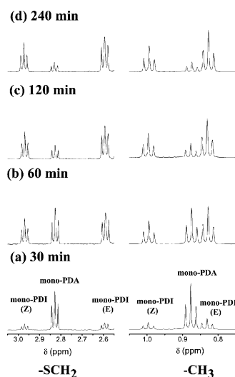
Fig. 13 The ^1\text{H} NMR monitoring of the redox reaction between PDI and mono-PDA in \text{DMSO-}d_6 at 70 °C.
