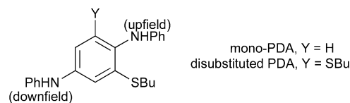
Fig. 9 The upfield and downfield phenylamino groups in the mono-PDA and 2,6-diPDA.
