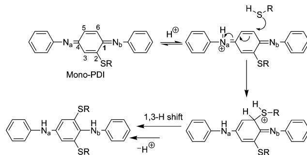
Fig. 10 Plausible mechanism for the preferential formation of 2,6-diPDA.
