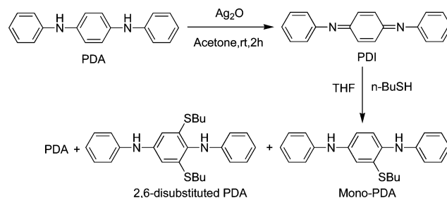
Scheme 1 CRS reaction of PDI with butane-1-thiol.
