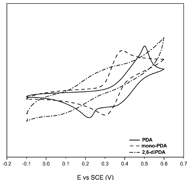
Fig. 14 The CV results of PDA, mono-PDA and 2,6-diPDA in an aqueous solution (pH = 1.3) containing 0.05 M TsOH.
