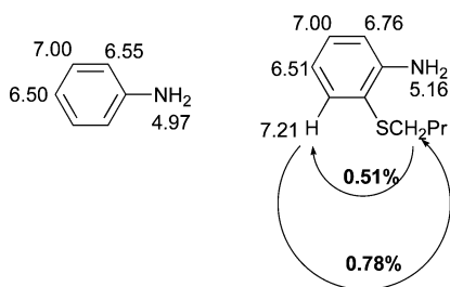
Fig. 1 The ^1\text{H} NMR chemical shift values ( \delta ppm) of aniline and 2-butylthioaniline and the NOE result for 2-butylthioaniline in \text{DMSO}-d_6 .
