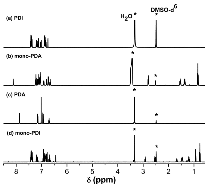
Fig. 12 The ^1\text{H} NMR spectra of (a) PDI, (b) mono-PDA, (c) PDA, and (d) mono-PDI in \text{DMSO-}d_6 .
