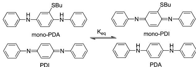
Fig. 11 The redox reaction between mono-PDA and PDI.
